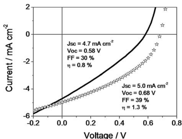
Fig. 9 J - V curves for photovoltaic cells illuminated at 100 \text{ mW cm}^{-2} (active area \approx 0.1 \text{ cm}^2 ), assembled with polymer/PCBM/CdSe (1 : 1 wt% PCBM : CdSe ratio, for nanoparticles with preferential diameter of 4.0 nm), using different polymers: (—) PFT or (☆) PF-PFT. The parameters extracted from the curves are shown.
