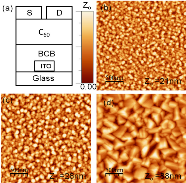
FIG. 1. (Color online) Schematic cross-section of OFET structures (a). AFM images of C_{60} films grown by flush evaporation at room temperature (b) and by HWE at a substrate temperature of 130 °C (c) and 250 °C (d).
