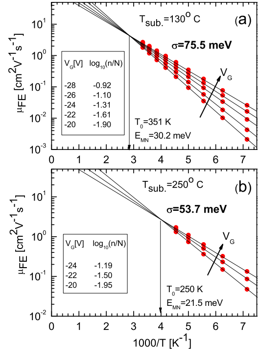
FIG. 2. (Color online) Temperature dependence of the OFET mobility measured at different V_G in C_{60} films grown by HWE at T_{sub}=130 °C (a) and 250 °C (b) (symbols) and results of their fitting with Eq. (2) (solid lines). The isokinetic temperature T_0 is indicated by an arrow.
