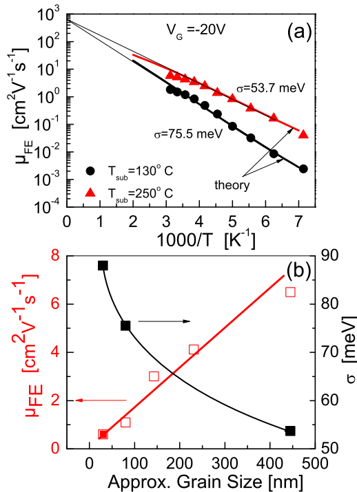
FIG. 3. (Color online) (a) Temperature dependence of the OFET mobility measured at constant V_G = -20 V in C_{60} films grown by HWE at T_{\text{sub}} = 130 °C and 250 °C (symbols) and results of calculated temperature dependences by the EMA theory (Ref. 12) (bold curves). Fitting experimental data with Eq. (2) is shown by thin solid lines. (b) Average OFET mobility in C_{60} films and width of the Gaussian DOS as a function of grain size in C_{60} films.
