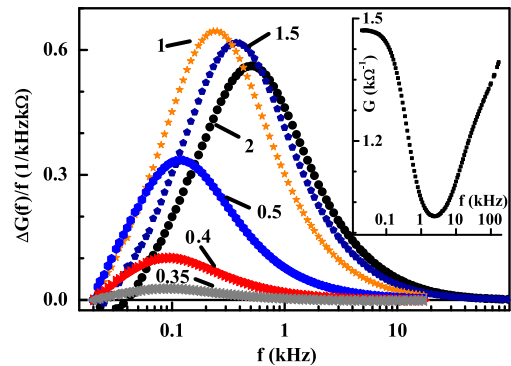
Fig. 2. The frequency dependence of \Delta G(f)/f \equiv [G(20 \text{ Hz}) - G(f)]/f for the same device as in Fig. 1, showing the typical bell shaped loss function behavior. Symbols: data points at various bias voltages (in V) as marked. Inset: G(f) vs f for V_{\text{bias}} = 1.5 V.
