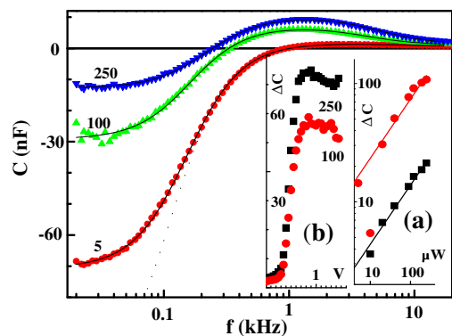
Fig. 3. The capacitance of the ITO-P3HT:PCBM-Al device vs frequency measured under laser illumination (532 nm) at I_L = 5, 100, 250 \mu\text{W} , as marked ( V_{\text{bias}} \approx 0.6 V). For clarity, only the frequency range 0.02–15 kHz is shown. Inset (a): the photoinduced changes \Delta C \equiv C_{\text{light}} - C_{\text{dark}} (in nF) at f = 50 Hz vs I_L (on a log–log plot) for V_{\text{bias}} = 0.35 (black square) and 0.5 V (red dots). The solid lines are fits to \Delta C \propto I_L^{1/2} law. Inset (b): \Delta C (in nF) at f = 50 Hz vs V_{\text{bias}} for I_L = 100 \mu\text{W} (red dots) and 250 \mu\text{W} (black square).
