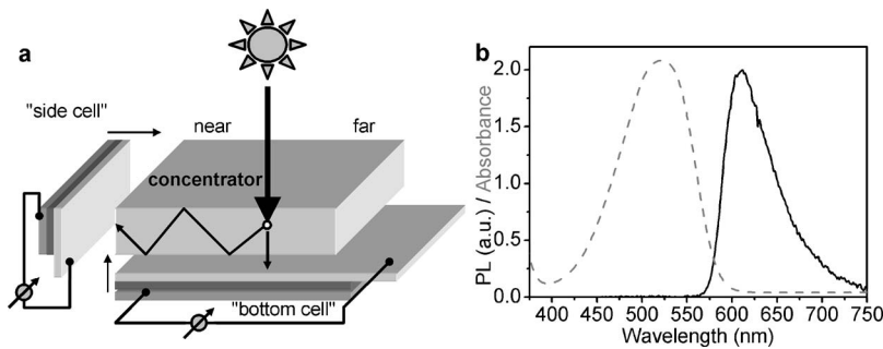
FIG. 1. (a) Schematic representation of the concentrator device. (b) Absorbance (dashed) and photoluminescence (solid) spectra of the concentrator plate.
