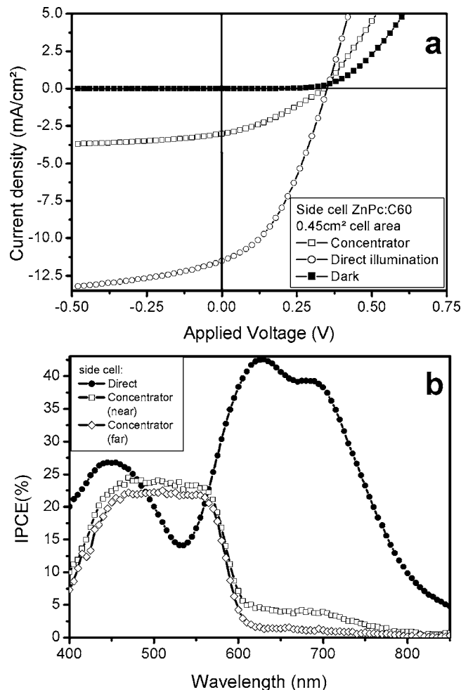
FIG. 2. (a) I - V characteristics of the side cell in the dark (solid squares), under direct 100 mW/cm 2 simulated AM1.5 illumination (open circles), and attached to the concentrator plate (open squares). (b) Incident photon to collected electron (IPCE) spectrum of the side cell under direct illumination (full circles) and attached to the concentrator plate [open squares: illumination close to the solar cell; open diamonds: illumination on the far side of the concentrator plate, as shown in Fig. 1(a)].
