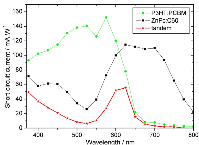
FIG. 2. (Color online) Current at short circuit condition vs wavelength of the incident monochromatic light for (■) the ZnPc/ZnPc: C_{60}/C_{60} individual cell, (●) the P3HT:PCBM diffused bilayer individual cell, and (★) the tandem cell.
