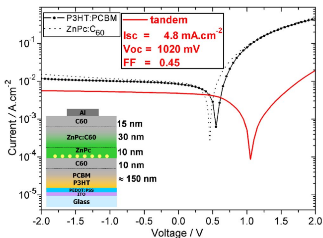
FIG. 1. (Color online) Current vs voltage of (dots) the ZnPc/ZnPc:C 60 /C 60 individual cell, (line plus symbol) the P3HT:PCBM diffused bilayer individual cell, and (full line) the tandem cell. The inset describes the structure of the tandem cell.
