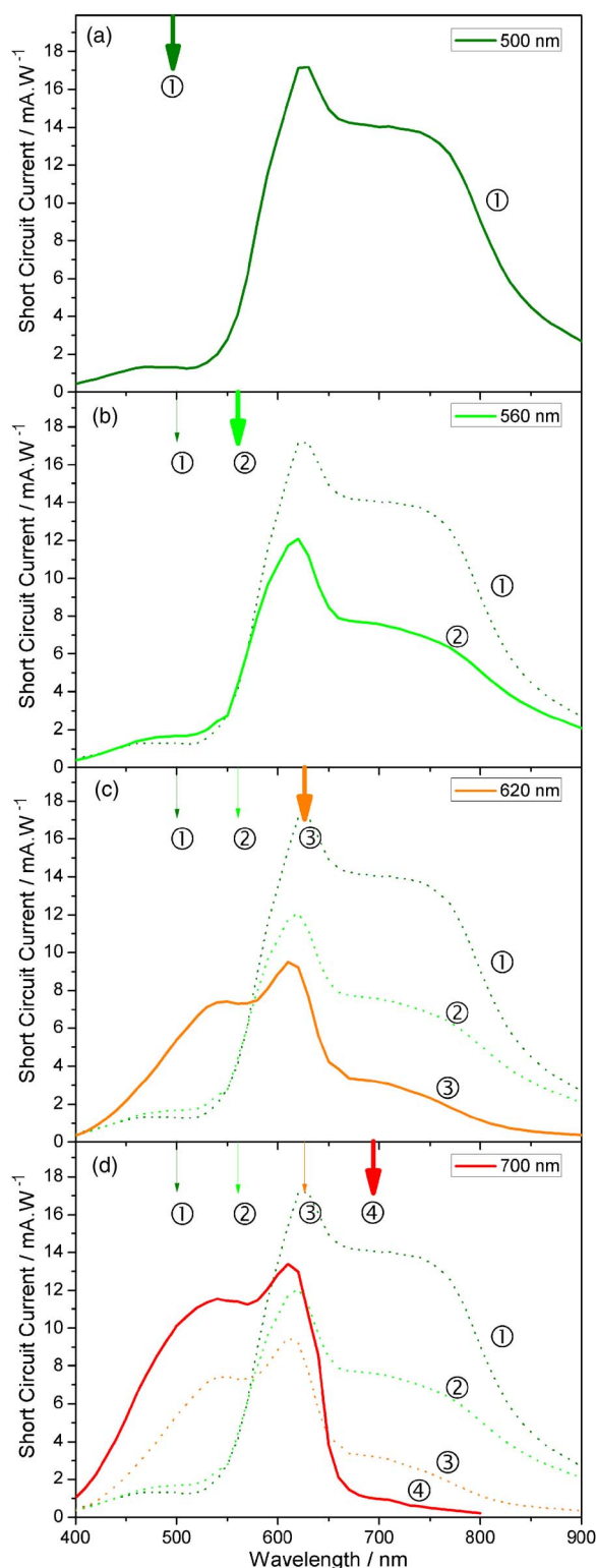
FIG. 3. (Color online) Current of the tandem device at short circuit condition vs wavelength of the incident monochromatic light. In this experiment, a second monochromatic nonchopped light source is used, the wavelength of which is indicated by the arrow: (a) 500 nm, (b) 560 nm, (c) 620 nm, and (d) 700 nm.
