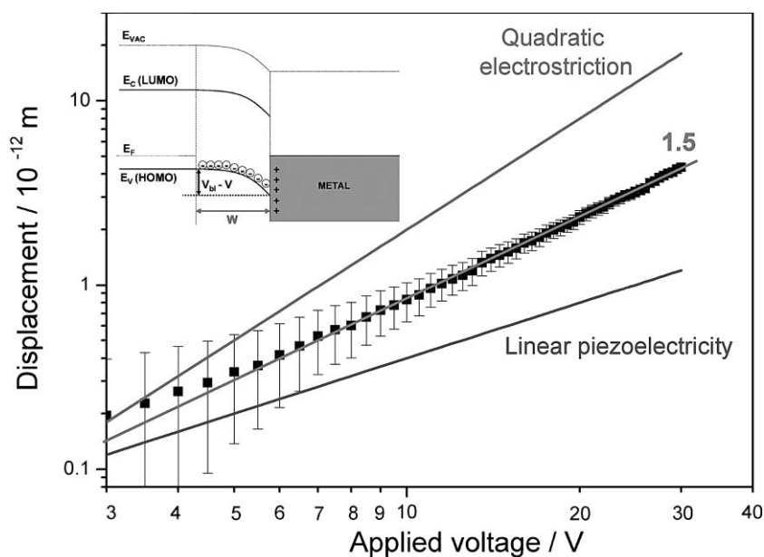
Fig. 4 Displacements recorded with a Nomarski interferometer on a Schottky ITO/P3HT/Al diode for reverse applied voltages (at 1555 Hz).
