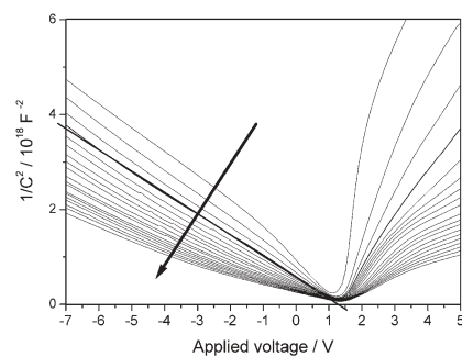
Fig. 3 1/C^2 of an ITO/P3HT/Al diode recorded at 1 kHz every 2 min in air versus the applied voltage V . The arrows indicate increasing time. The thick solid line is a linear fit of one intermediate curve.
