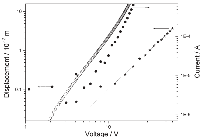
Fig. 2 Electromechanical displacement of the upper surface of a ITO/MDMO-PPV/Al diode versus the amplitude of the sinusoidal voltage (at a frequency of 33.3 Hz) in forward (●) and reverse direction (★). Each curve is fitted by a power law: The exponents found are respectively 4.4 (●) and 2 (★). Right axis: Current through the diode (○) in forward direction.
