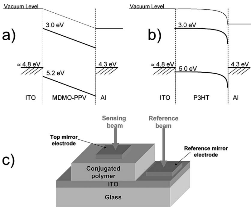
Fig. 1 Energetic diagram of (a) undoped MDMO-PPV and (b) p-doped P3HT sandwiched between ITO and Al. In (a), the electric field is homogeneous throughout the entire device thickness while in (b), the field drops linearly in the depletion zone present in the polymer on the Al side. (c) Schematic cross-section of a diode designed to allow Nomarsky interferometer measurements.
