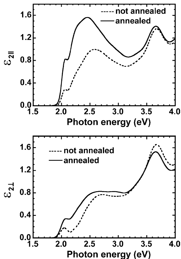
Fig. 3. Parallel (upper panel) and perpendicular (lower panel) components of the imaginary part of the anisotropic dielectric function of the untreated (dashed line) and the annealed (solid line) P3HT/PCBM-films.
