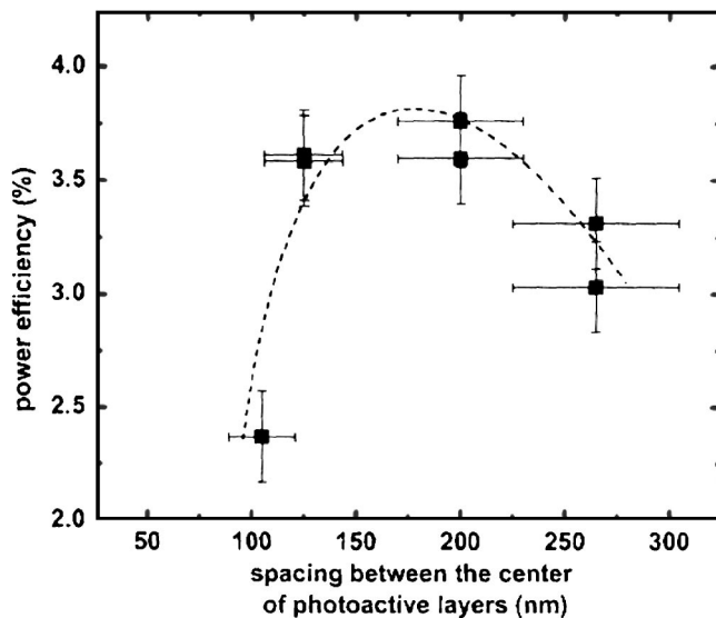
FIG. 3. Power efficiencies for p-i-n tandem cells plotted vs the distance between the centers of the photoactive layers. The device structure has been kept constant except for the separating hole transport layer between Cells A and B. The dashed line represents a guide for the eyes.
