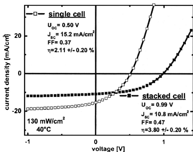
FIG. 2. I-V characteristics of single and tandem p-i-n solar cells under 130 \text{ mW/cm}^2 simulated AM 1.5 solar illumination. The tandem cell has an optimized device structure according to the simulation shown in Fig. 1, and the single cell is identical to the bottom cell in the tandem configuration (Cell A) prepared simultaneously. The performance parameters are given.
