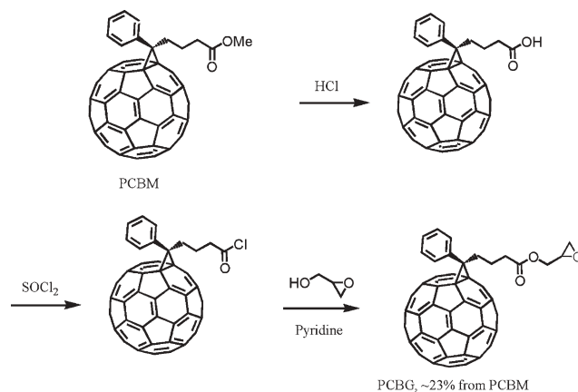
Scheme 1 Synthesis of C 61 -butyrac acid glycidol ester (PCBG).
