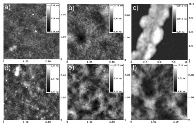
Fig. 1 AFM images of P3HT–PCBM (a–c) and P3HT–PCBG (d–f) blend films spin cast on glass. The images show unheated films (a and d), films annealed for 4 min at 140 °C (b and e), and films annealed for 1 h at 140 °C (c and f).
