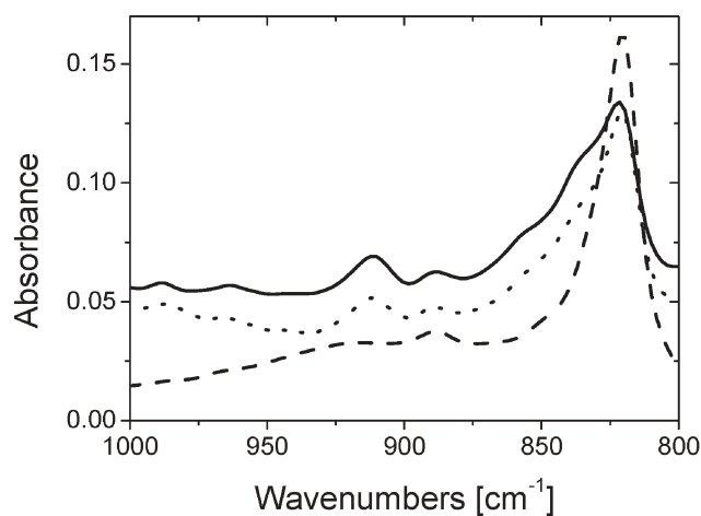
Fig. 6 IR absorption spectra of a P3HT-PCBG-initiator film before (solid) and after (dotted) heating at 140 °C for 1 h. For reference a pristine P3HT film is shown (dashed).
