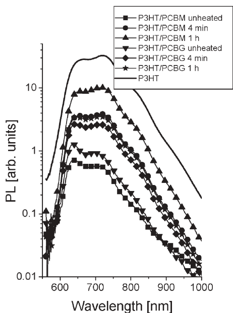
Fig. 3 Photoluminescence spectra of unheated and heated P3HT–PCBM and P3HT–PCBG blend films. In the unheated blend films the PL is quenched by two orders of magnitude compared to the pristine polymer. In the heated films the PL increases slightly compared to the unheated films.
