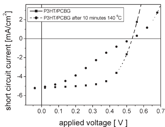
Fig. 7 Current-voltage curves measured under illumination (AM 1.5 simulated, 80 \text{mW cm}^{-2} ). Squares, P3HT-PCBG device after production and post treatment, circles, P3HT-PCBG device after an additional thermal treatment (10 min, 140 °C).
