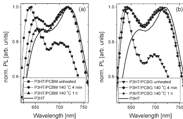
Fig. 4 Normalized PL spectra of unheated and heated P3HT–PCBM (a) and P3HT–PCBG (b) films. While the unheated blend films show their maximum PL around 640 nm and a second peak at 700 nm, the pristine polymer has its maximum PL at 720 nm and a smaller peak around 667 nm. The heated P3HT–PCBM films show PL peaks that shift with longer heating times from the unheated to the pristine polymer peak positions. The heated P3HT–PCBG films show two peaks of about the same magnitude, one of them close the maximum PL of the unheated blends and one close to the maximum of the pristine polymer film. The heating time does not influence the shape of the PL in the case of P3HT–PCBG films.
