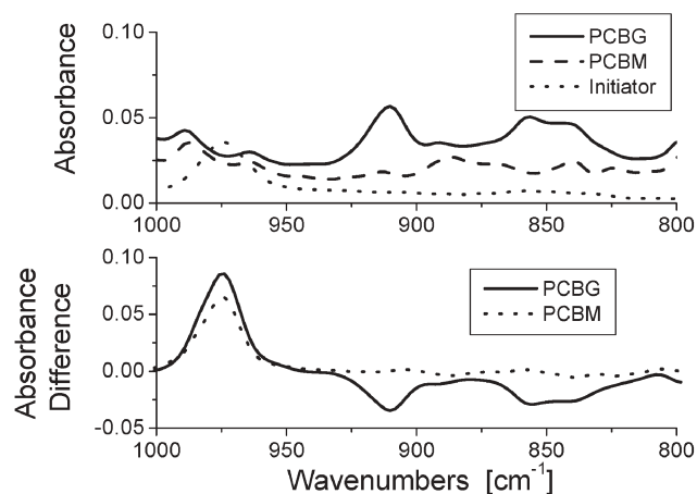
Fig. 5 IR absorption spectrum of a PCBG, a PCBM and a tris(pentafluorophenyl)borane film (top) and IR absorption difference spectra of PCBG and PCBM before and after addition of the initiator (bottom).
