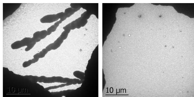
Fig. 2 TEM images of a P3HT–PCBM film (left) and a P3HT–PCBG film (right), both annealed at 140 °C for 1 h. While the PCBM has phase separated into large crystals, the PCBG does not show any large scale phase separation.
