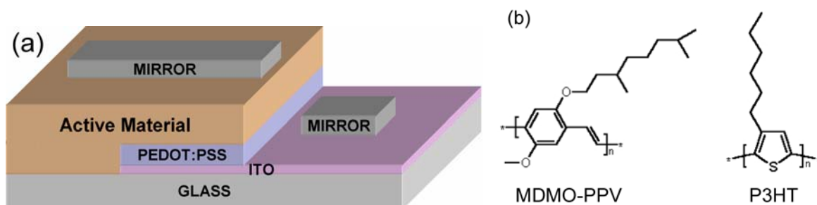
Figure 1: (a) Structure of the conjugated polymer based diode; (b) Chemical structure of the two active materials exploited, namely poly-[2-(3,7-dimethyloctyloxy)-5-methyloxy]-para-phenylene-vinylene (MDMO-PPV) and poly(3-hexyl-thiophene) (P3HT).
