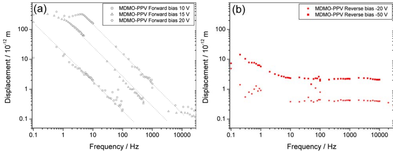
Figure 4 : Electromechanical strain recorded at the surface of a MDMO-PPV diode under (a) forward and (b) reverse polarization.
