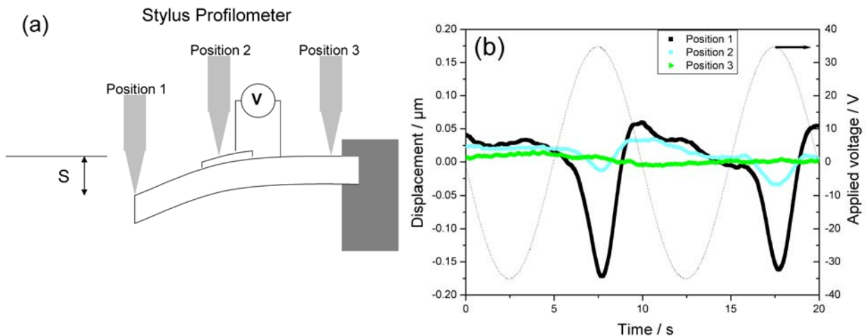
Figure 5 : Displacement measured at (a) different points of the glass substrate (b) versus applied voltage.
