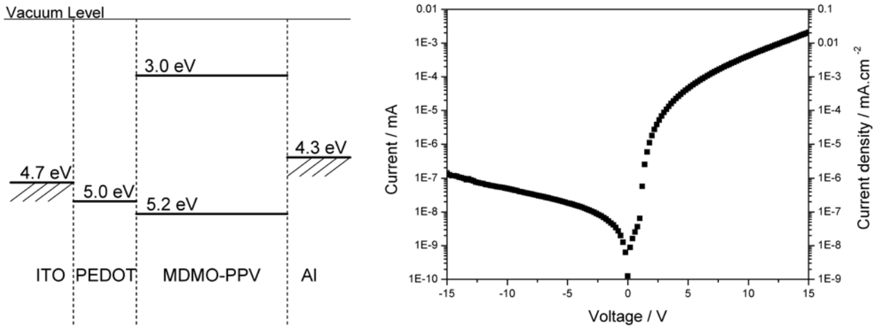
Figure 2 : (a) Energetic level diagram of the MDMO-PPV based diodes according to the MIM picture; (b) Current versus voltage graph of a MDMO-PPV diode (active surface area of 0.1 cm 2 ).
