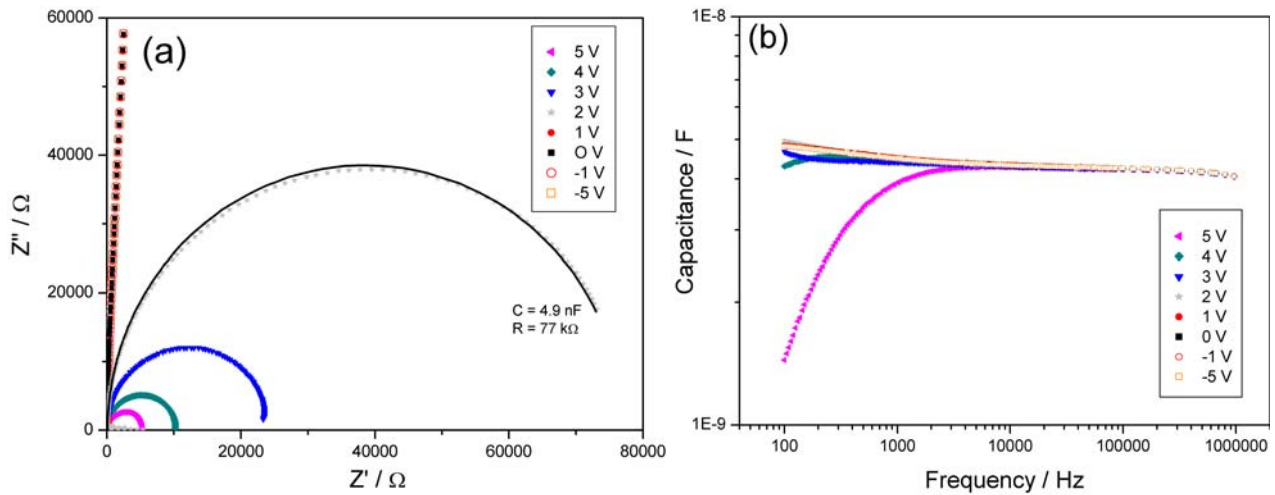
Figure 3 : (a) Cole-Cole diagram and (b) capacitance versus frequency of a MDMO-PPV diode (thickness:150 nm; surface area: 0.2 cm 2 ) under different applied voltages.
