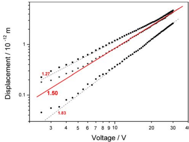
Figure 7 : Displacement versus voltage applied for a doped P3HT diode.
