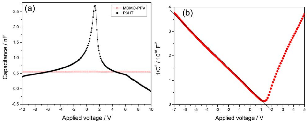
Figure 6 : (a) Capacitance versus voltage performed at 1 kHz on MDMO-PPV and P3HT diodes ; (b) 1/C^2 plotted versus voltage for the P3HT case.
