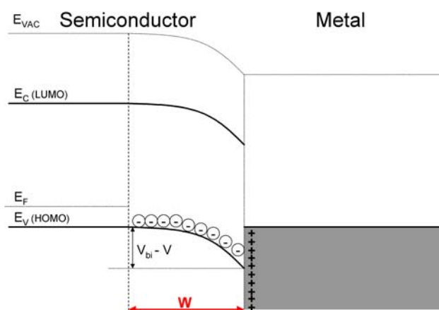
Figure 8 : Energy diagram of a Schottky contact.
