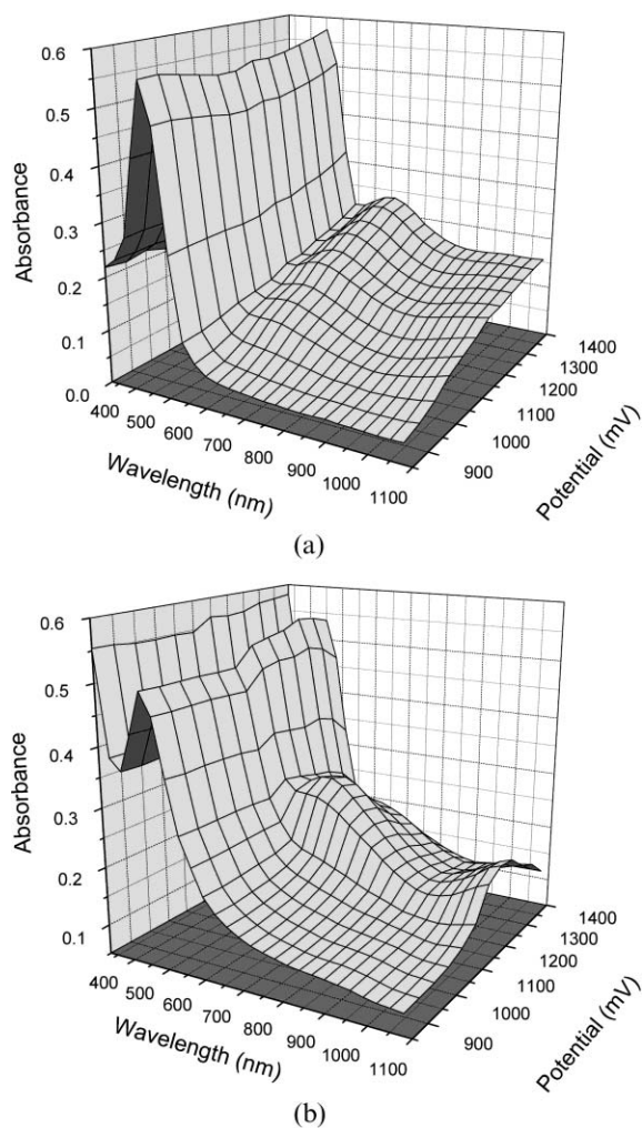
Fig. 4 UV-vis spectroelectrochemical measurements of (a) 10a and (b) 10b on ITO glass.
