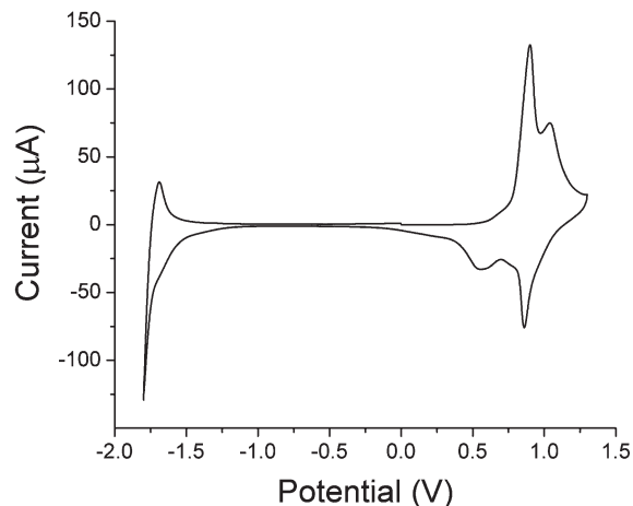
Fig. 2 Cyclic voltammogram of compound 10a as a spin-coated film on ITO glass, under identical conditions to those presented in Fig. 1.
