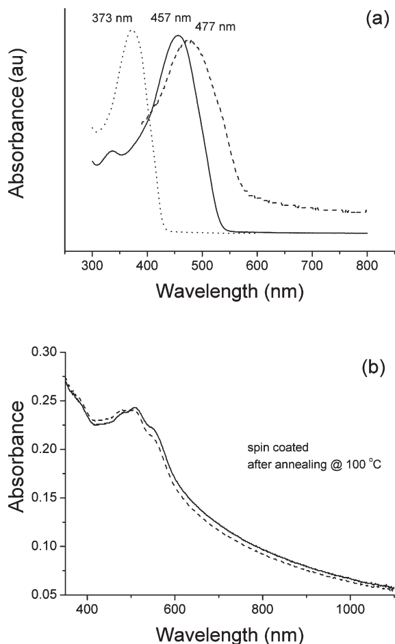
Fig. 3 Absorption spectra of (a) compounds 9a (···) and 10a (—) in dichloromethane solution and 10a (---) as a film on ITO glass, and (b) compound 10b as a film on ITO glass.
