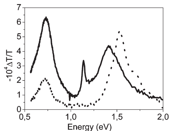
Fig. 6 Photoinduced absorption spectra of mixed layer 10a :C 60 (—) and pure 10a (···) solid films. Excitation at 476 nm, T = 18 K.
