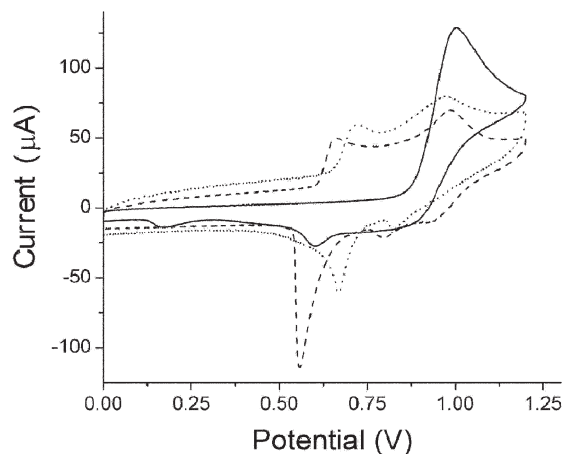
Fig. 1 Cyclic voltammograms of compounds 9a (—), 10a (---) and 10b (···) in CH 2 Cl 2 vs. Ag/AgCl reference electrode, Au disk working electrode, TBAPF 6 as the supporting electrolyte (0.1 M), substrate concentration 10 -3 M, scan rate 100 mV s -1 .
