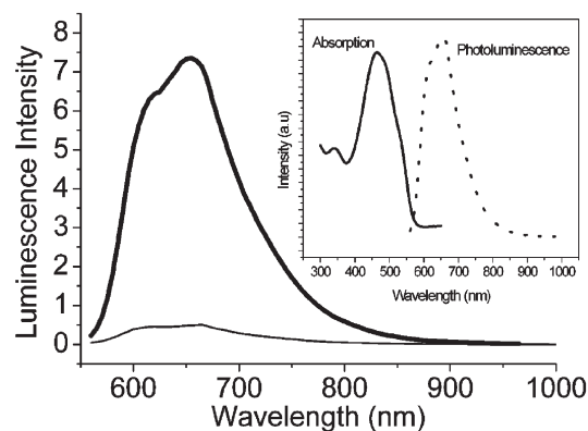
Fig. 5 Photoluminescence spectra in blends of 10a and C 60 (—) and 10a film (---). The electron transfer to C 60 quenches the photoluminescence of 10a . Inset: Absorption (—) and photoluminescence (···) spectra of pristine 10a .
