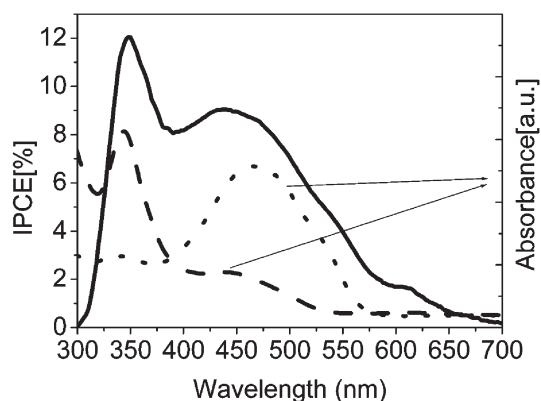
Fig. 8 IPCE characteristics of the bilayer device using ITO/PEDOT| 10a (40 nm)| C_{60} (60 nm)|Al (—) is compared with the absorption spectra of 10a (---) and C_{60} (···).
