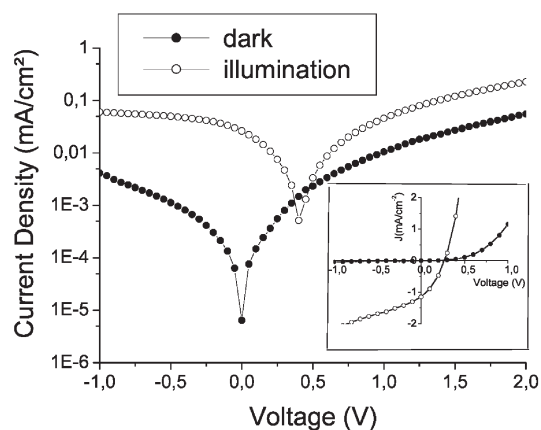
Fig. 7 Logarithmic and linear (inset) representations of the current density–voltage characteristics of a 10a | C_{60} cell. The empty circles represent data obtained under 100 \text{ mW cm}^{-2} white light illumination while the full circles represent data measured in the dark.
