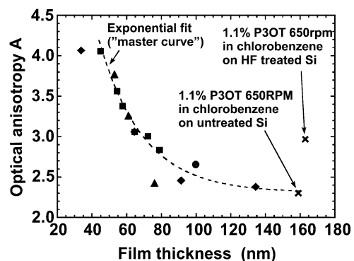
Fig. 3. Anisotropy parameter A of spin-coated P3OT-films prepared by: various spin frequencies (750, 1000, 1500, 2000, 3000, 4000 rpm) on untreated Si substrates from 1.1% chlorobenzol solution (■); various polymer concentrations (0.7, 1.1, 1.5, 2.0%) on untreated Si substrates from chlorobenzene solution by 1500 rpm (◆); various spin frequencies (2000, 3000, 4000 rpm) on glass substrates from 1.5% chlorobenzol solution (▲); 1500 rpm on Si substrate from 1.1% toluene solution (●). The experimental points fall closely on a single 'master curve', an exponential decay.
