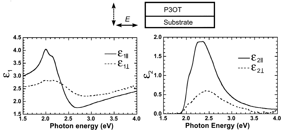
Fig. 1. Real \varepsilon_1 and imaginary \varepsilon_2 parts of the parallel (solid line) and perpendicular (dashed line) components of the anisotropic DF of spin-coated P3OT-films prepared by 3000 rpm from a 1.5% chlorobenzene solution (film thickness 61 nm).
