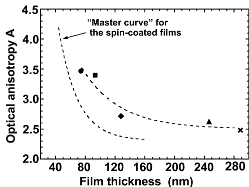
Fig. 4. Anisotropy parameter A of drop-cast P3OT-films prepared from: 0.7% chlorobenzene solution on glass (●); 0.7% chlorobenzene solution on untreated Si (■); 1.1% toluene solution on untreated Si (◆); 1.5% chlorobenzene solution on glass (▲); 1.5% chlorobenzene solution on untreated Si (×). The 'master curve' for spin-coated films (in this figure) is also shown for comparison.
