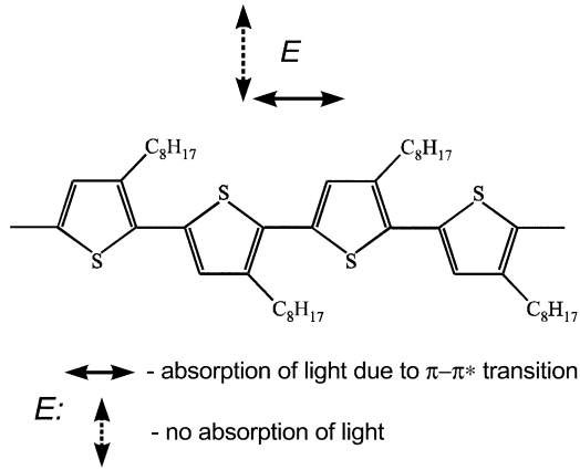
Fig. 2. Chemical structure of P3OT. E is the vector of electric field. The lowest in energy \pi - \pi^* transition is polarized parallel to the polymer backbone. No absorption occurs for the light polarized perpendicular to the main chain (in the spectral range considered here).
