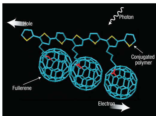
Figure 1 Photoinduced charge transfer in a polymeric material composed of a conjugated moiety with covalently linked fullerene-based units 3 . The structure is designed to behave as a semiconducting double-cable: the conjugated polymer (unsaturated backbone) allows for the transport of holes (p-type conduction), whereas the tethered fullerene units allow for the transport of electrons (n-type conduction). Roncali and colleagues 1 have now created a three-dimensional polymeric fullerene structure, which also behaves as an intrinsic p/n-type semiconductor with enhanced stability and tunable morphology. (Yellow: sulphur. Blue: carbon. Red: nitrogen.)
