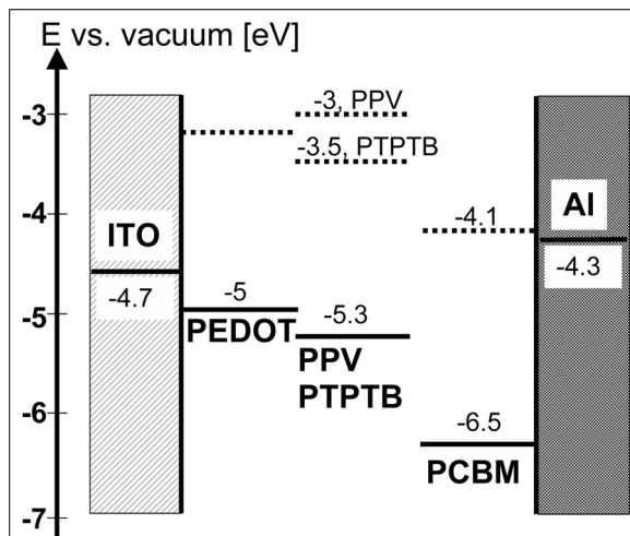
FIGURE 7 Energy diagram for an organic solar cell with the determined values for the HOMO \blacksquare and the LUMO \dashv ; values for PCBM taken from literature [13], for PEDOT value for “Baytron” from the Bayer company.
