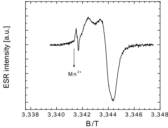
Figure 3. ESR spectrum of iodine-doped MDMO-PPV, represented as a function of the magnetic field B . The signal Mn^{2+} was used for calibration.
