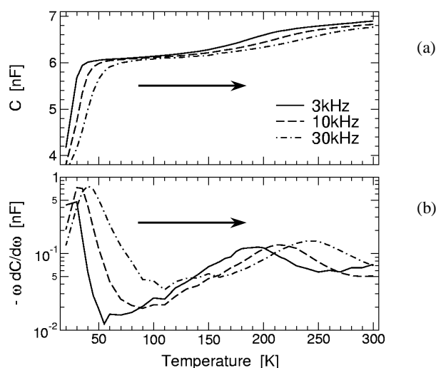
Figure 5. (a) Capacitance C as a function of the temperature T for different frequencies. (b) Differentiated -\omega dC/d\omega versus T for different frequencies. The arrows indicate the direction of increased frequency.
