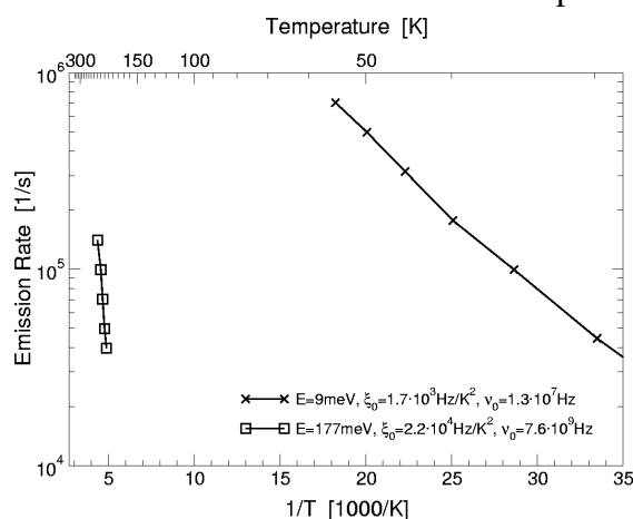
Figure 6. Arrhenius evaluation of the admittance spectra of an ITO/PEDOT:PSS/MDMO-PPV:PCBM/Al device. Two different, frequency-dependent contributions to the device capacitance were found at activation energies E_{A1}=9 meV and E_{A2}=177 meV.
