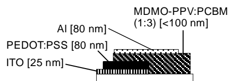
Figure 1. Device configuration for a bulk-heterojunction photovoltaic device with the structure ITO/PEDOT:PSS/ MDMO-PPV:PCBM/Al. The thickness of the different layers is displayed in brackets.
