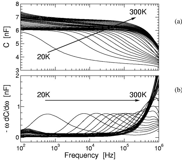
Figure 4. (a) Frequency spectrum of the device capacitance C(\omega) of a ITO/PEDOT:PSS/MDMO-PPV:PCBM/Al solar cell. The arrows indicate the direction of increasing temperature. (b) Normalised derivative -\omega dC/d\omega of the capacitance-frequency spectrum C(\omega) .
