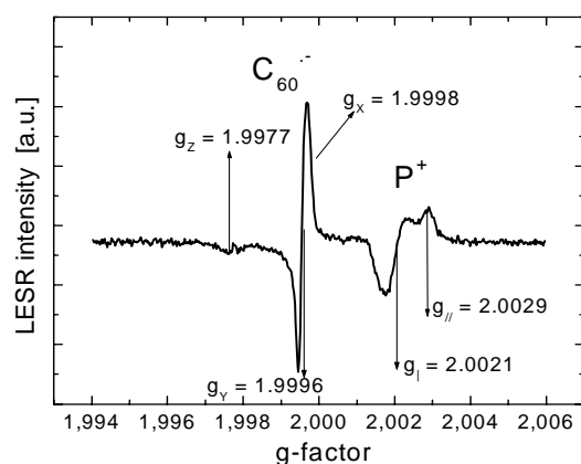
Figure 2. W-band LESR spectrum for a composite of MDMO-PPV and PCBM. Two different line groups are resolved and attributed to the polymer cation P^+ and to the anion of the C_{60} derivative PCBM.
