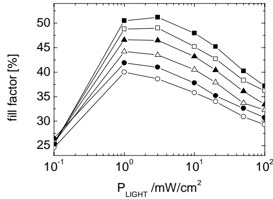
Figure 3. Fill factor as a function of illumination intensity. The temperature varied from 100 K (open circles) to 300 K (full squares) with steps of 40 K.
