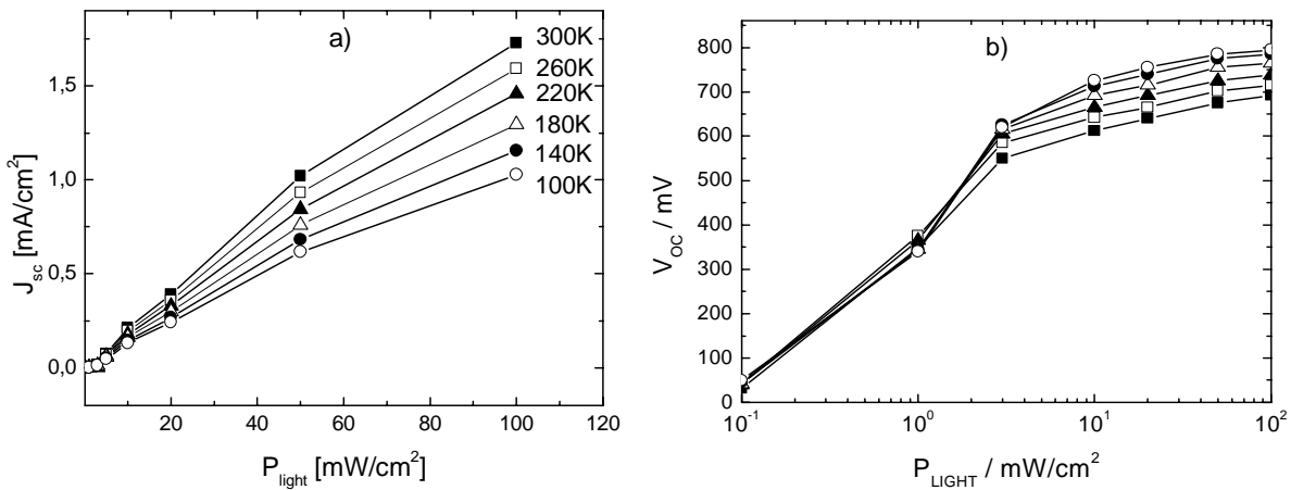
Figure 2. a) Short-circuit current density J_{SC} as a function of illumination intensity. The temperature varied from 100 K to 300 K;
