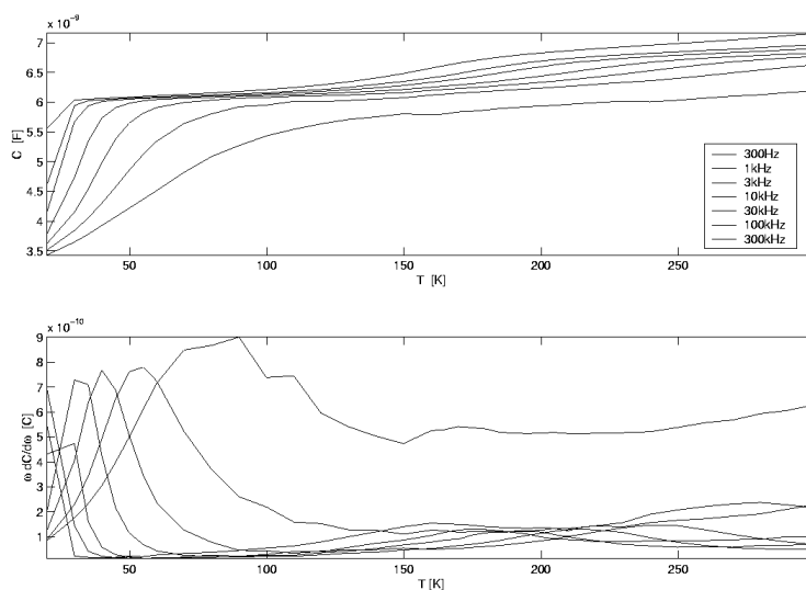
Figure 7. Capacitance (upper graph) and differentiated capacitance (lower graph) vs. temperature at different frequencies (indicated).
