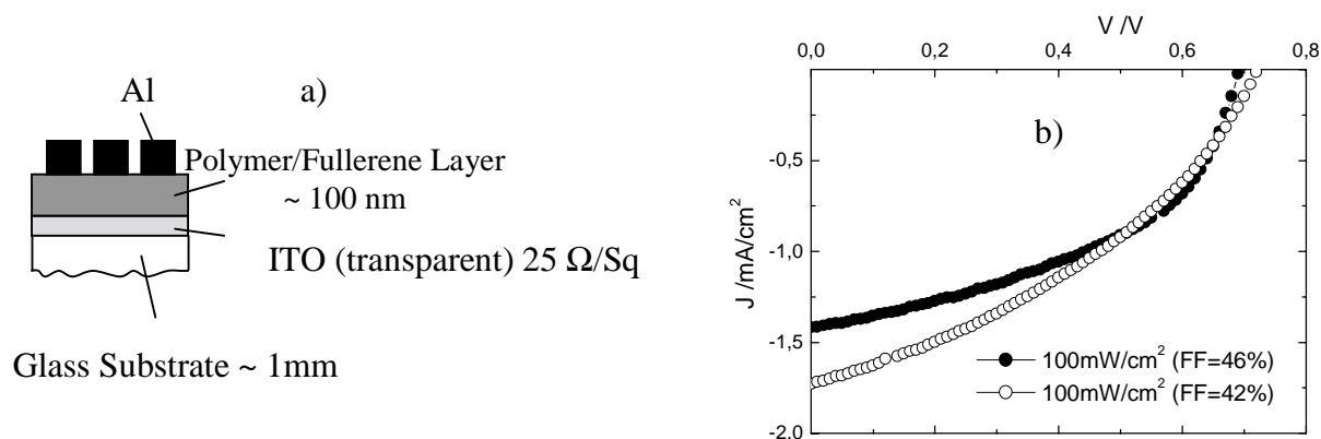
Figure 1. a) Configuration for of a ITO/MDMO-PPV:PCBM/Al device. (A layer of the doped conducting polymer PEDOT:PSS between ITO and the composite was added, but it is optional.); b) Current-voltage characteristics for two devices with different fill factors.
