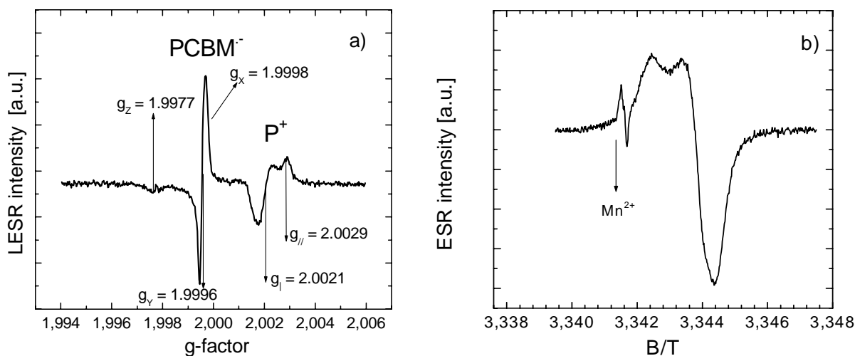
Figure 9. a) LESR spectrum of the MDMO-PPV/PCBM composite, showing the methanofullerene anion radical PCBM - and the positive polaron P + . T=100 K, \lambda_{exc.}=488 nm.; b) ESR ("dark") spectrum of I 2 -doped MDMO-PPV. T=100 K.
