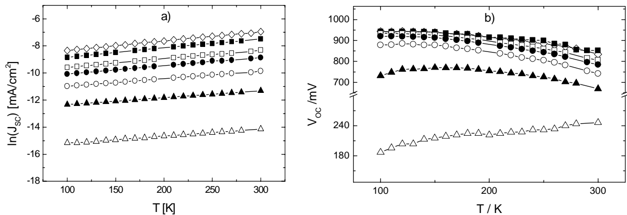
Figure 4. a) Temperature dependence of the short-circuit current density J_{SC} . The symbols correspond to different illumination intensities: 0.1 mW/cm^2 (open triangles), 1 mW/cm^2 (full triangles), 3 mW/cm^2 (open circles), 10 mW/cm^2 (full circles), 20 mW/cm^2 (open squares), 50 mW/cm^2 (full squares), 100 mW/cm^2 (open diamonds); b) open circuit voltage as a function of temperature.
