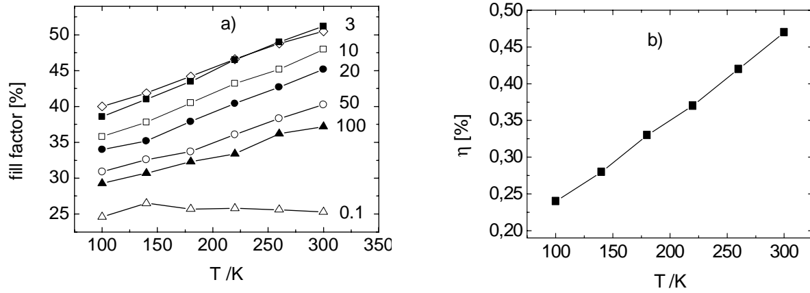
Figure 5. a) Fill factor vs. temperature for different intensities (in \text{mW}/\text{cm}^2 ); b) Power conversion efficiency vs. temperature. The device was illuminated with white light of 100 \text{ mW}/\text{cm}^2 .
