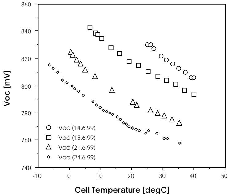
Fig. 3: Open-circuit voltage (Voc) vs. cell temperature, during outdoor tests, 14-24 June 1999.
