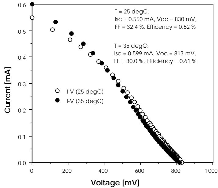
Fig. 6: I-V curves at T = 25 \text{ }^\circ\text{C} and T = 35 \text{ }^\circ\text{C} for the first outdoor tests (June 14, 1999).
