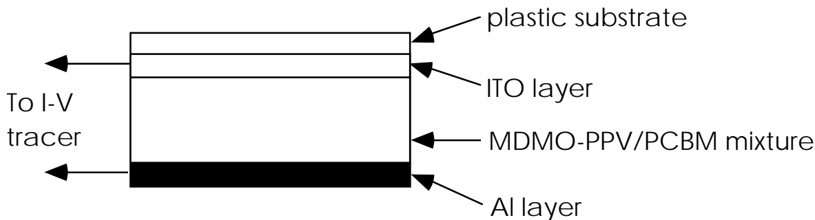
Fig. 1: Schematic device structure of the fullerene/conjugated polymer solar cells under study.
