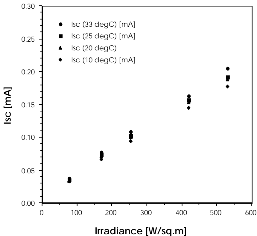
Fig. 2: Short-circuit current (Isc) vs. Irradiance level, at various cell temperatures.
