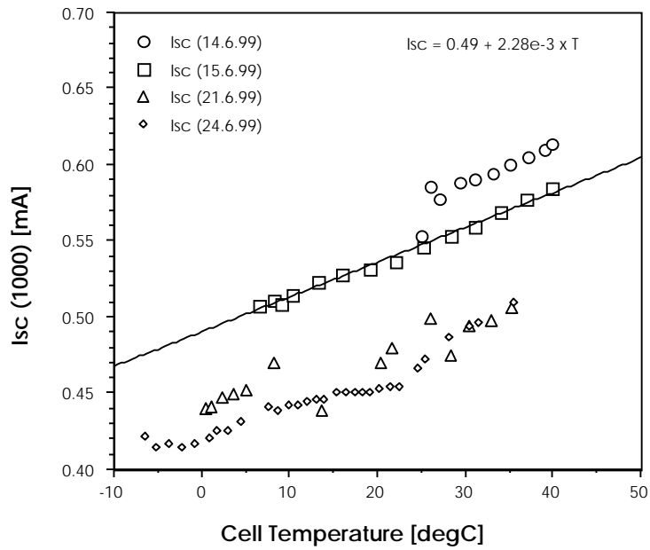
Fig. 4: Isc (adjusted to irradiance 1000 \text{ W m}^{-2} ) vs. cell temperature during outdoor tests 14-24 June 1999.
