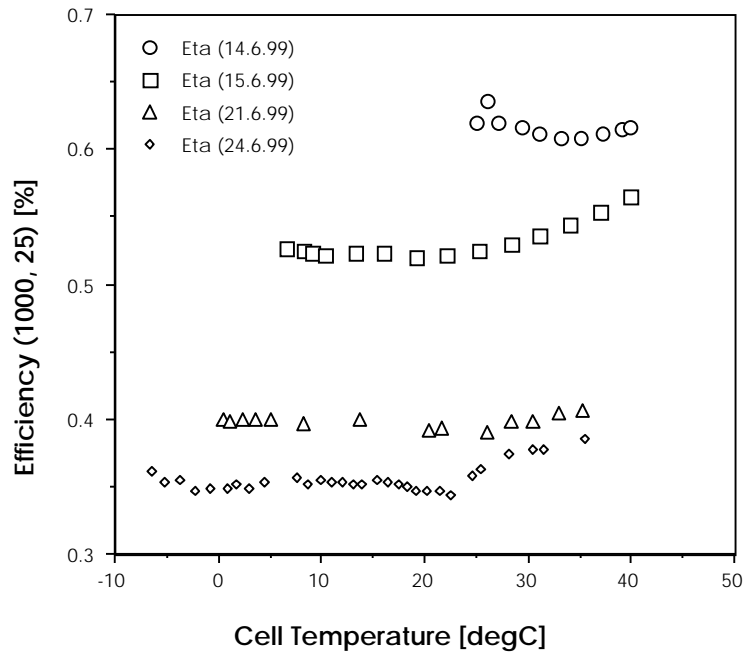
Fig. 5: Efficiency \eta (adjusted to irradiance 1000 \text{ Wm}^{-2} ) vs. cell temperature, during outdoor tests 14-24 June 1999.
