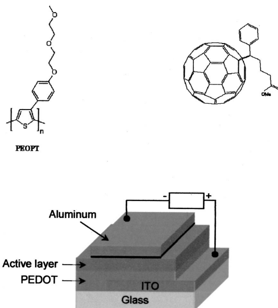
FIG. 1. Chemical structure of PEOPT and PCBM and solar cell device structure.
