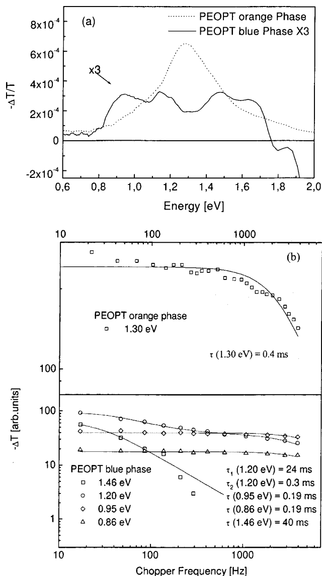
FIG. 3. (a) PIA spectra of PEOPT in the blue (continuous line) and orange phase (dotted line) at 80 K and 10^{-3} Pa, excitation at 488 nm with 150 mW laser power for the blue phase and 30 mW for the orange phase, chopper frequency 122 Hz. (b) Frequency dependence of the PIA features ( \Delta T ) of PEOPT in the orange phase at 1.30 eV (open square, upper part) and for PEOPT in the blue phase at 1.46 eV (open square), at 1.20 eV (open circle), at 0.95 eV (open diamond), and 0.86 eV (open triangle) for PEOPT blue phase (lower part). The continuous lines are fits to a monomolecular decay model. The experimental conditions were as denoted in (a).
