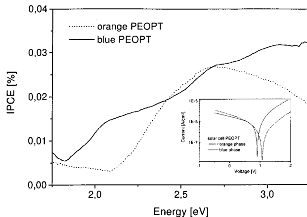
FIG. 6. Spectrally resolved photocurrent of blue PEOPT (continuous lines) vs orange PEOPT (dotted lines). The inset shows the I - V curves under white light illumination with 60 mW/cm 2 . Under these conditions, the following values were measured for the blue phase, V_{oc} =0.91 V, I_{sc} =1.9 \mu A/cm 2 , FF=0.30, and for the orange phase, V_{oc} =1.06 V, I_{sc} =2.2 \mu A/cm, FF=0.24.
