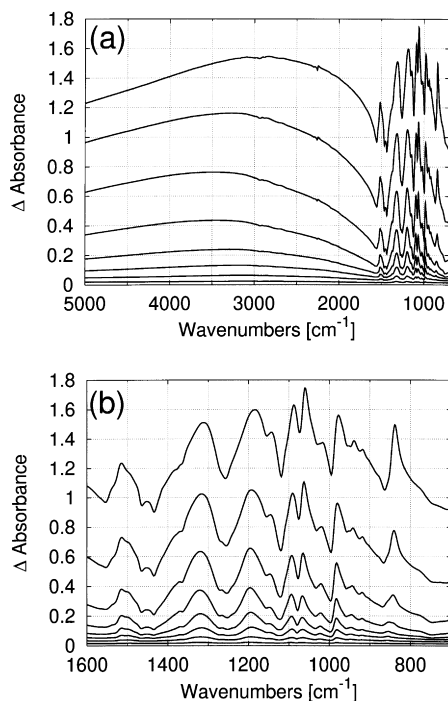
Fig. 3. In situ FTIR-ATR difference spectra of a PEDOT film in 0.1 M TEAPF 6 -acetonitrile solution during anodic potential sweep (p-doping) between -900 and +600 mV; scan rate 5 mV/s; reference spectrum at -900 mV. (a) full spectral region; (b) enlargement of (a) in the region 1600 – 700 cm -1 .
