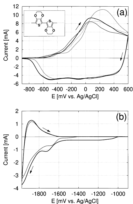
Fig. 2. Cyclic voltammograms of a PEDOT film on a Pt electrode cycled in 0.1 M TBAClO 4 -acetonitrile solution at a scan rate of 100 mV/s. Thick lines: first cycle; thin lines: second cycle. (a) p-doping of a fresh film (solid lines), p-doping after n-doping (dotted lines); (b) n-doping between the p-doping experiments. Inset: structure of PEDOT.
