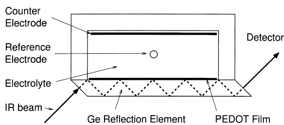
Fig. 1. Setup of the spectroelectrochemical cell.
