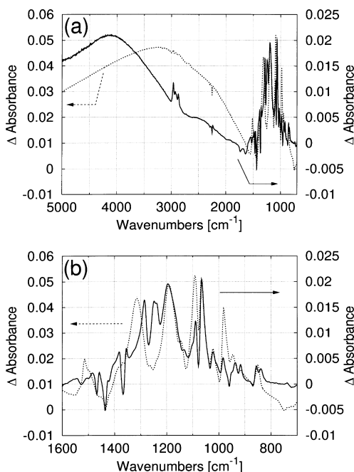
Fig. 6. Comparison of in situ FTIR-ATR difference spectra of p-doped and n-doped PEDOT with similar doping levels in 0.1 M \text{TBAClO}_4 -acetonitrile solution. Solid line: n-doped, spectrum at -1800 mV, reference spectrum at -1500 mV; dashed line: p-doped, spectrum at -300 mV, reference spectrum at -900 mV. (a) full spectral region; (b) enlargement of (a) in the region 1600 – 700 \text{cm}^{-1} .
