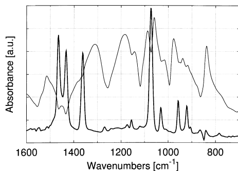
Fig. 4. In situ spectrum of a neutral PEDOT film at -900 mV (thick line, reference spectrum: filled cell without polymer), and the spectrum of a p-doped film at +500 mV (reference spectrum at -900 mV). The spectra are separated and scaled individually.
