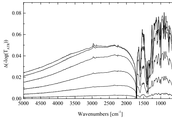
Figure 3. Difference in situ ATR-FTIR absorption spectra during reduction process A for potentials from -95 mV to -618 mV. Reference spectrum taken around -48 mV.
