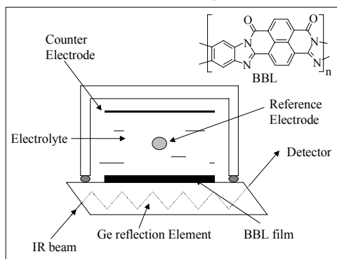
Figure 1. In situ ATR-FTIR spectroelectrochemical cell. Inset: BBL chemical structure.
