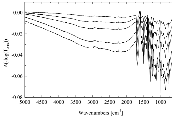
Figure 4. Difference in situ ATR-FTIR absorption spectra during reduction process B for potentials from -618\text{ mV} to -1039\text{ mV} . Reference spectrum taken around -572\text{ mV} .
