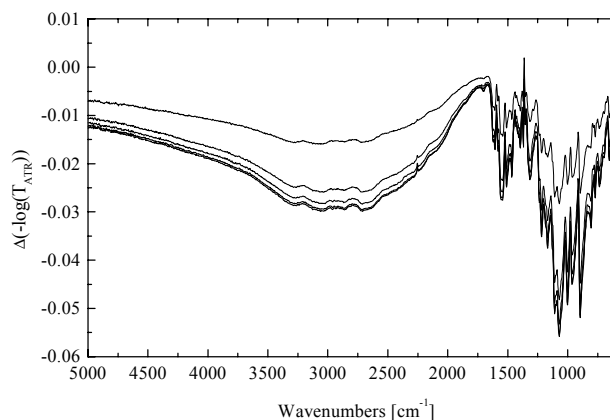
Figure 6. Difference in situ ATR-FTIR absorption spectra during reduction process D for potential from -1206 mV to -1634 mV. Reference spectrum taken around -1164 mV.
