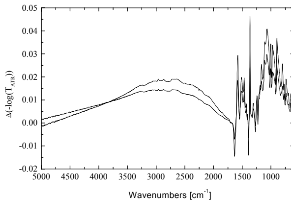
Figure 5. Difference in situ ATR-FTIR absorption spectra during reduction process C for potential from -1039 mV to -1206 mV. Reference spectrum taken around -996 mV.
