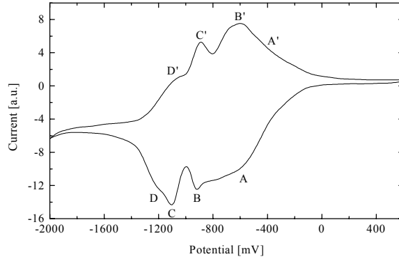
Figure 2. CV for n -doping (reduction) processes of BBL.
