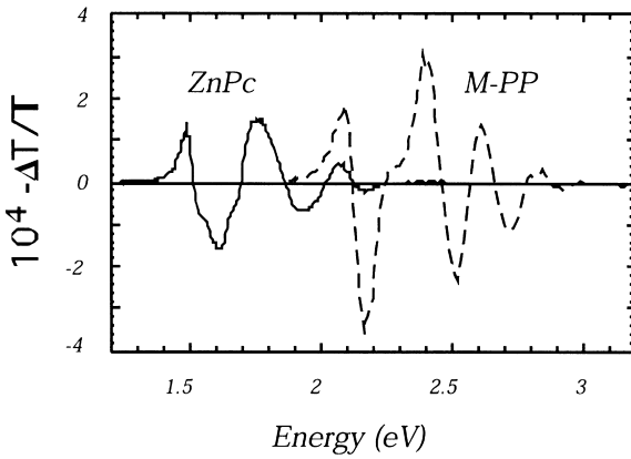
Fig. 2. The electroabsorption spectra of ZnPc (solid line) and MPP (dashed line).
