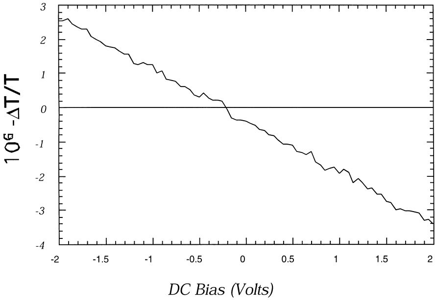
Fig. 4. The EA response of the MPP device vs. DC bias.
