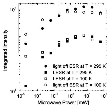
FIG. 9. Saturation behavior of the LESR signal (full squares ■) and of the light-off ESR signal (full circles ●) at 295 K and of the LESR signal (open squares □) and of the light-off ESR signal (open circles ○) at 100 K. Light-off signal was taken after LESR measurement switching off illumination.
