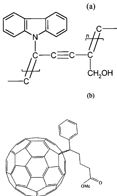
FIG. 1. Chemical structure of (a) polyCPDO and (b) PCBM.
