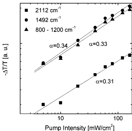
FIG. 5. Intensity dependence of -\Delta T/T for excitation power at 488 nm at 2112 \text{cm}^{-1} (C \equiv C, full squares \blacksquare ), 1492 \text{cm}^{-1} (C=C, full circles \bullet ) and for the integral over 800–1200 \text{cm}^{-1} (full triangles \blacktriangle ). The lines are fits with a power law -\Delta T/T \sim I_{488}^\alpha , where the exponent \alpha turns out to be \sim 0.31 , \sim 0.33 , and \sim 0.34 for the three spectral regions.
