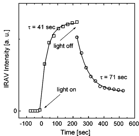
FIG. 6. Rise (open squares \square ) and decay (open circles \circ ) behavior of the photoinduced absorption -\Delta T/T at 100 K during and after illumination with laser light at 488 nm with 25 \text{mW}/\text{cm}^2 . Fits with exponential growth and decay behavior yielded 41 s for the rise time \tau_1 and 71 s for the relaxation time \tau_2 , respectively. For the relaxation behavior the -\Delta T/T signal was evaluated by integrating over the IRAV region between 800 and 1200 \text{cm}^{-1} . Similar time constants were obtained from the C \equiv C IRAV band.
