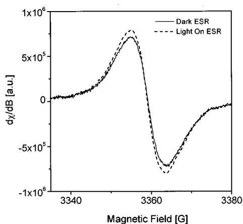
FIG. 7. Dark ESR (—) and light-on ESR (---) signal of polyCPDO at 100 K and 2 mW microwave power.
