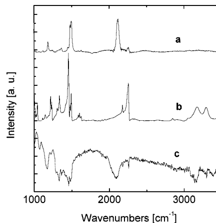
FIG. 4. Raman spectrum (a), IR absorption (b), and IRAV (c) of polyCPDO after UV polymerization.
