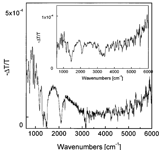
FIG. 3. -\Delta T/T for microcrystalline polyCPDO in pressed KBr pellets. The inset shows -\Delta T/T for a polyCPDO/PCBM composite, produced by drop casting of monomer solution onto KBr pellets and UV polymerization.
