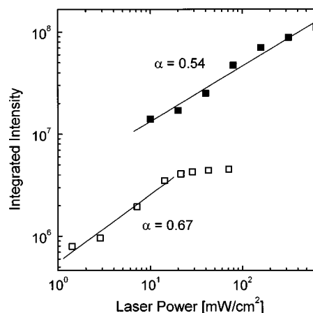
FIG. 10. Light intensity dependence of LESR signal of polyCPDO at 100 K (□) and 295 K (■). Power law fits of the type y=x^\alpha yield exponents \alpha=0.67 at 100 K and \alpha=0.54 at 295 K.
