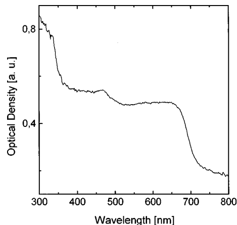
FIG. 2. Absorption spectrum of polyCPDO, polymerized by UV light.
