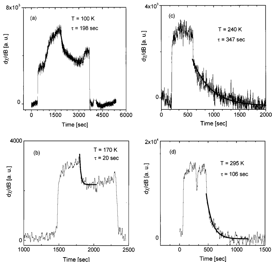
FIG. 11. Slow dynamics of photoexcited spins in polyCPDO for four temperatures: (a) T=100 K, (b) T=170 K, (c) T=240 K, and (d) T=295 K. Illumination was provided by the 488 nm line of an argon ion laser at a power of 25 mW/cm 2 . Relaxation times were fitted by exponential decay law, fits are drawn as full lines in the figures.
