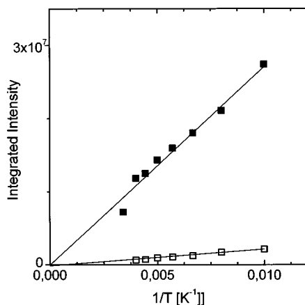
FIG. 8. Temperature dependence of the integrated intensity of the microwave absorption of the dark signal (full squares ■) and of the LESR signal (open squares □). Lines are extrapolations to a 1/T fit.
