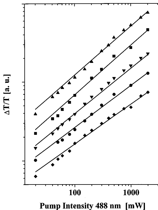
FIG. 10. Intensity dependence of the low C_{60} sample peak at five different positions from 1.4–1.7 eV. Lines are nonlinear fits with a power law y = a \cdot x^\alpha . The following data have been calculated: 1.4 eV [full karo (◆)], \alpha = 0.50 , 1.47 eV [full circles (●)], \alpha = 0.54 , 1.5 eV [full down triangles (▼)], \alpha = 0.57 , 1.61 eV [full squares (■)], \alpha = 0.63 , 1.69 eV [full up triangles (▲)], \alpha = 0.62
