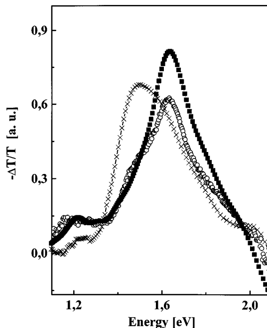
FIG. 9. -\Delta T/T for PS/MEH-PPV samples with low [crosses (x)], intermediate [hollow circles (○)] and high C_{60} [full squares (■)] concentration at 80 K and 10^{-5} Torr. The energetic position of the peaks are 1.51 eV for the low concentrated system and 1.63 eV for the intermediate and high concentrated system.
