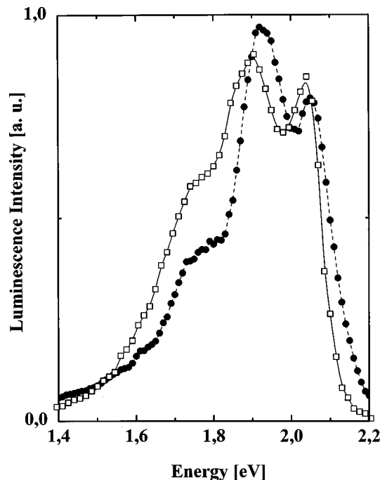
FIG. 4. Luminescence data of PE/MEH-PPV composites with [hollow squares (□)] and without [full circles (●)] PC 61 BCR at 80 K and 10 -5 Torr. The weight ratio between MEH-PPV and PC 61 BCR is 1:2. For the oriented sample the 488 nm pump beam is parallel to the stretch direction.
