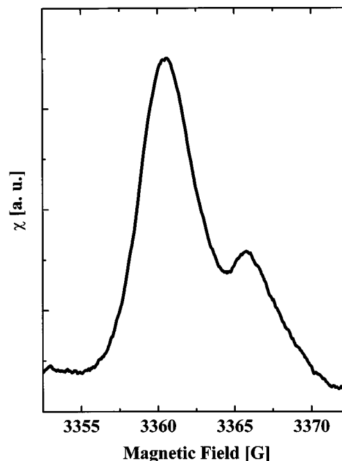
FIG. 13. Integral of LESR spectrum [full line (—)] of the concentrated PS/MEH-PPV/ C_{60} compound presented in Fig. 12. Evaluation of the signal yields two peaks, one at low magnetic fields with a g value of g=2.0023 and one at higher fields with a g value of g=1.9997 . Signals are interpreted as MEH-PPV^+ polaron and C_{60}^- anion, respectively.
