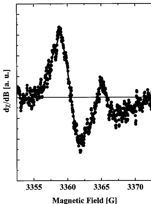
FIG. 12. LESR spectrum [full circles (●)] of the concentrated PS/MEH-PPV/ C_{60} compound with equal weight ratios. The line represents data after smoothing by a Savitzky Golay filter. LESR spectrum is recorded at 100 K and 10^{-4} Torr as the difference between the illuminated signal and the signal after switching off the light. Illumination is provided through a 50% grid by 70 mW of the 488 nm line of an Ar^+ laser. Microwave power is 2 mW. Prior to illumination samples are heated up to room temperature to relax long living radicals and cooled down to 100 K.
